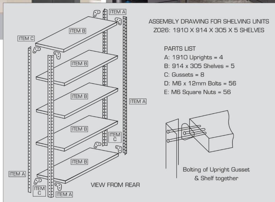
Z026 ASSEMBLY INSTRUCTIONS
